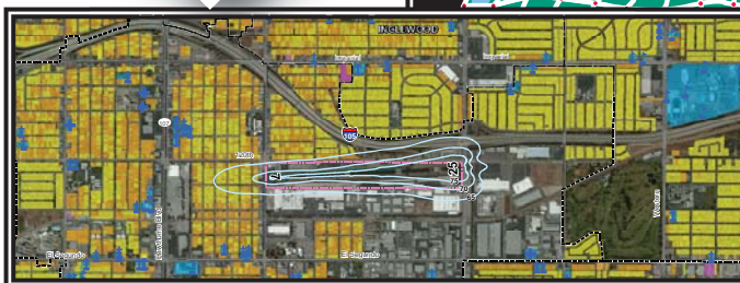
Noise Contours
